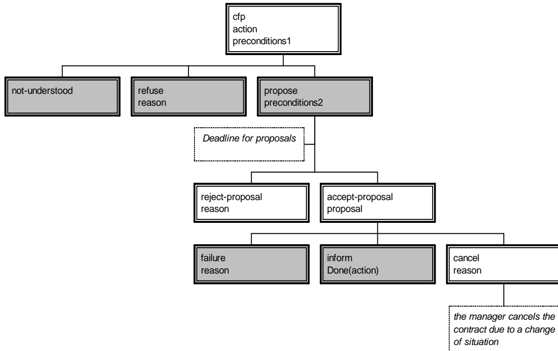
Figure 6 - FIPA-Contract-Net Interaction Protocol
