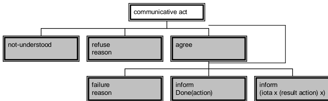
Figure 5 - Homogeneous structure of the interaction protocols.
