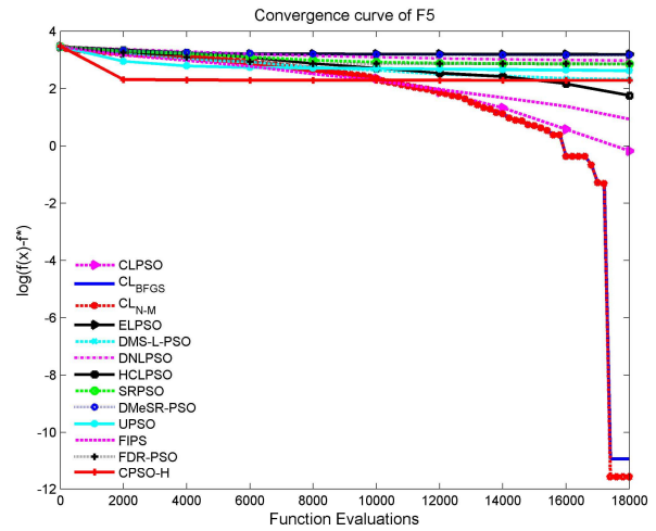
Fig. 5. Convergence curve of different PSO variants for 10-D F5.
