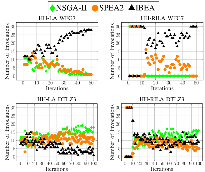
Fig. 6. Number of invocations of each MOEA at each iteration over 30 trials on WFG7 and DTLZ3 obtained from HH-LA (left column) and HH-RILA (right column).
