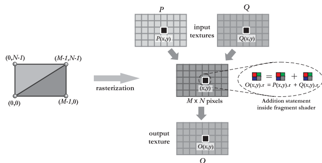
Figure 2: Addition of two matrices on GPU.
