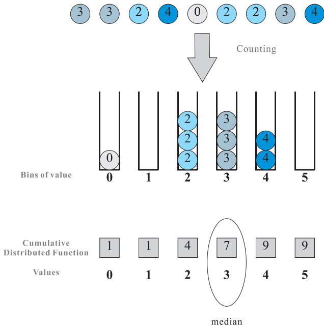
Figure 6: Running example of median picking algorithm.
