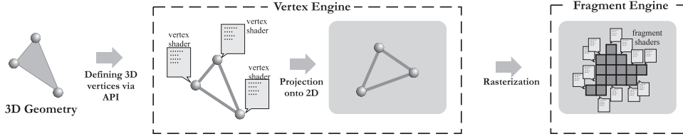
Figure 1: The 3D rendering pipeline.
