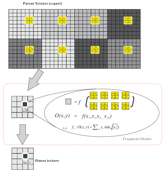
Figure 5: The shader for fitness evaluation.
