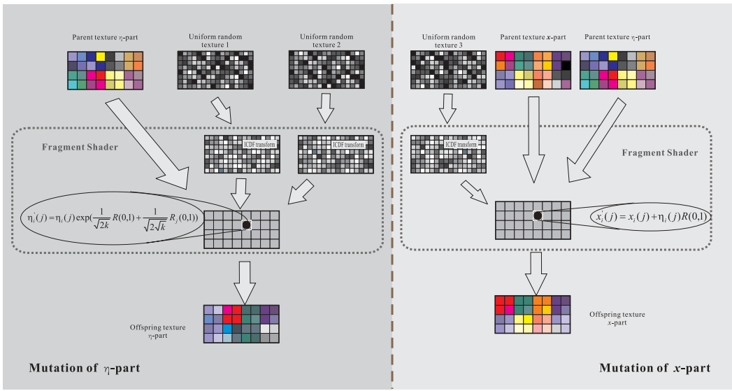
Figure 4: The two fragment shaders for mutation process.
