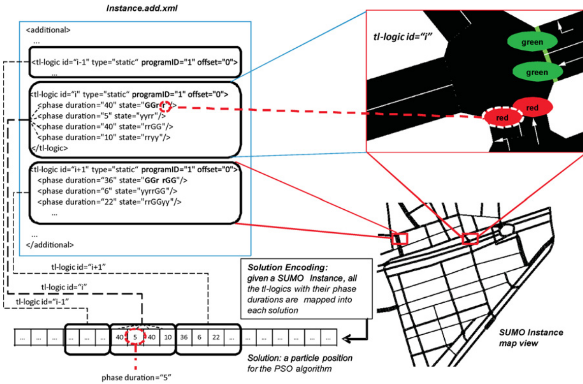
Fig. 1. Intersection with four traffic lights selected from the SUMO instance map. Phase durations (cycles) are specified in the instance.add.xml file and encoded inside a PSO tentative solution.
