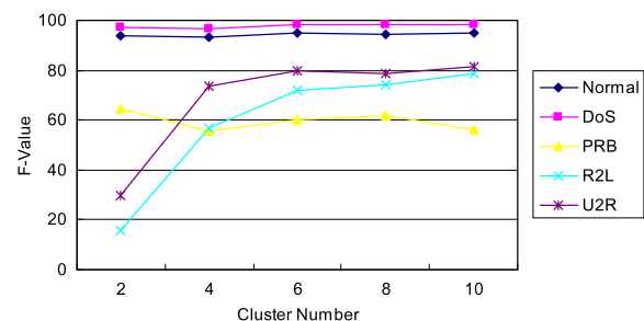
Fig. 7. F-value (%) of different clustering number.
