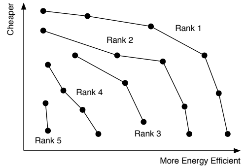
Figure 51 Pareto ranks.
