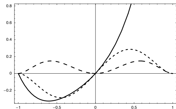
Figure 71 The functions f(x) : —, g(x) : ---, and h(x) : -.- as discussed in the Symbolic Regression section. f(1) = 4 .
