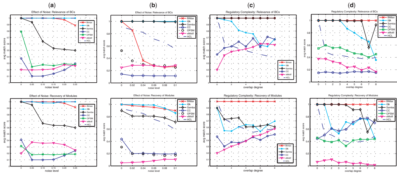
Fig. 2. Results for the artificial scenarios: non-overlapping modules with increasing noise levels for (a) constant and (b) additive biclusters, overlapping modules with increasing overlap degree and no noise for (c) constant and (d) additive biclusters. Note that OPISM is excluded in (c), cf. results section.
