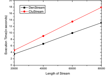
Figure 15: Execution time vs. length of stream(Charitable Donation data set)
