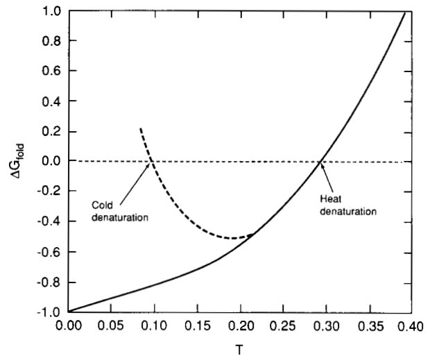
Fig. 23. Free energy of folding \Delta G_{fold} (in units of |\epsilon| ) versus temperature T (in units of |\epsilon|/k ) for HP sequence studied by Gupta and Hall (1995), where \epsilon is a constant (continuous curve). Sequence is shown in its unique native structure in Figure 24C (ii). Curvature in \Delta G_{fold} is caused by shifting subpopulations in the denatured ensemble, as in HTM. Dashed curve indicates that cold denaturation would occur if |\epsilon| decreases with decreasing temperature.
