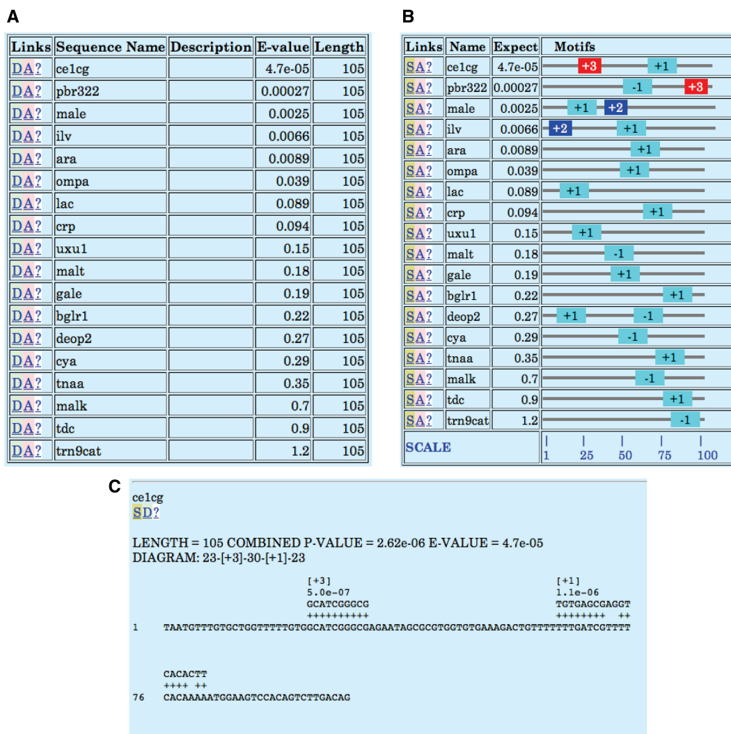
Figure 6. MAST output. The figure shows the result of searching with three MEME motifs against 18 E. coli DNA sequences containing the CRP binding site. The MAST output contains three representations of the results, excerpts of which are shown in the three figure panels. The E -value score of the overall match of the motif(s) in the input is shown in the first results section (Panel A). The second section (Panel B) displays the relative locations of significant matches of the motifs in the sequences. The third results sections gives a detailed picture of the motif matches, showing the exact location and p -value score of each motif match aligned above the target sequence.
