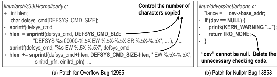
Figure 3. R2Fix automatically generated the two patches, both of which have been accepted and committed to the code repository by the kernel developers after we reported them. The generated patches are directly applicable to the faulty code, but are simplified for illustration.
