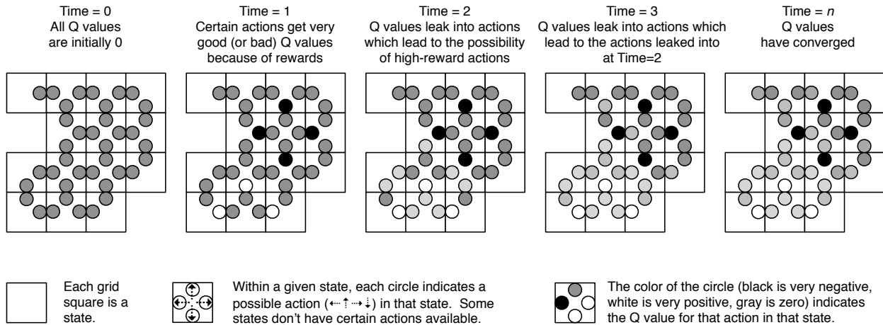
Figure 65 Illustration of Q-Learning with a model in the cockroach robot world. By time= n , the best (lightest color) action in each state corresponds to the optimal policy action in Figure 63.
