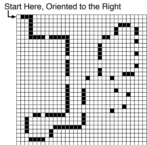
Figure 71 The Santa Fe Trail, a toroidal grid world. Black squares indicate pellet locations.
