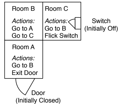
Figure 67 A robot world with three rooms, a door, and a switch. available actions for each room are shown. The robot can only exit if the door is opened. Flicking the switch opens the door.
