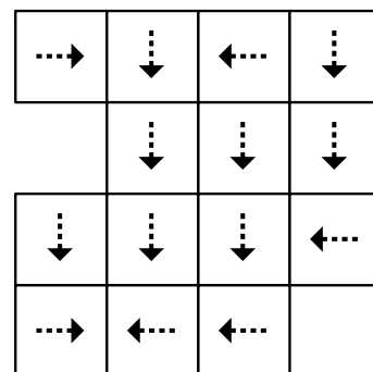
Figure 63 An optimal policy for the cockroach robot world.
