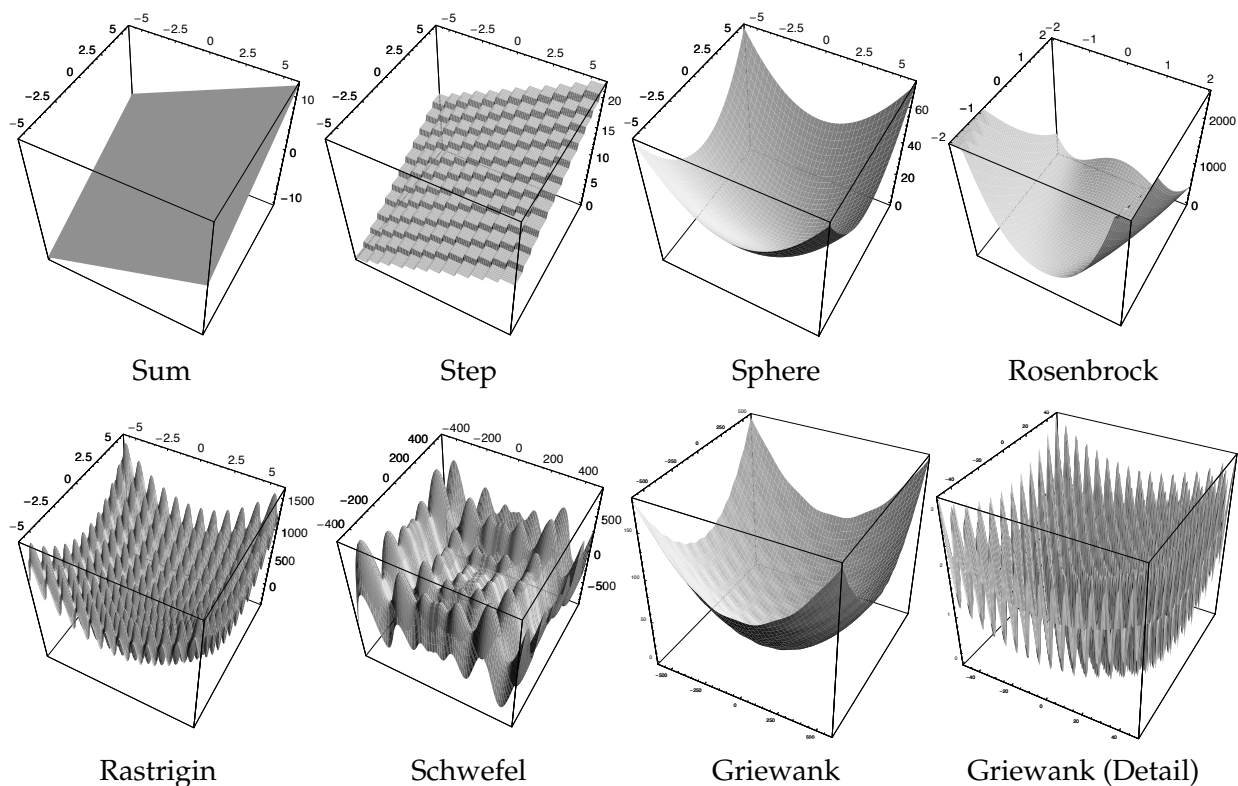
Figure 68 Real-valued problems in two dimensions ( \langle x_1, x_2 \rangle ).
