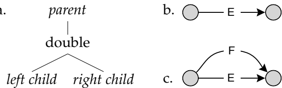
Figure 23 The double Edge Encoding operator.
