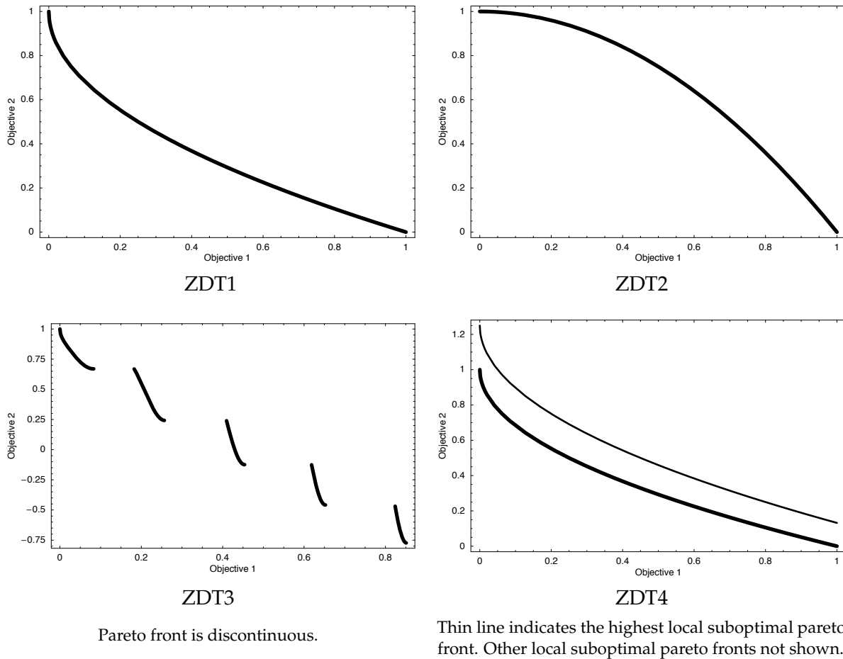
Figure 69 Pareto fronts of four multiobjective problems (ZDT1, ZDT2, ZDT3, and ZDT4) as described in Section 11.2.3. All four problems are minimization problems, so lower objective values are preferred.
