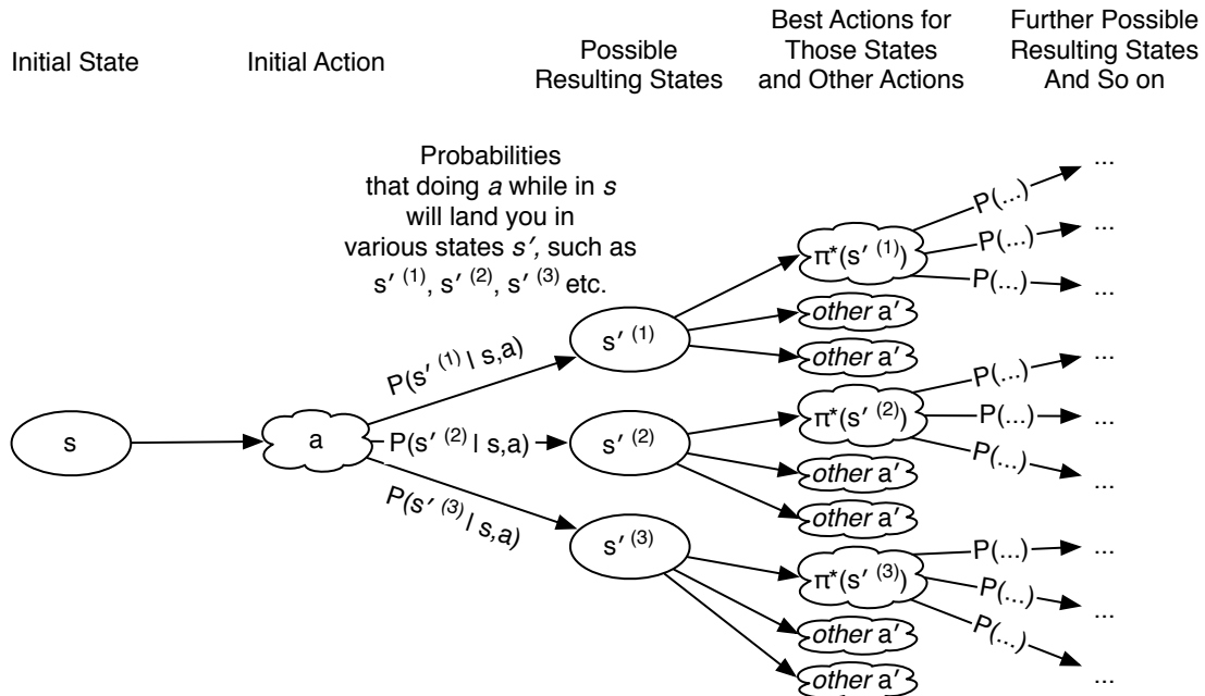
Figure 64 The Q-Learning state-action model. We are presently in some state s and decide to perform an action a . With a certain probability P(s'|s, a) , doing that action a while in s leads to a state s' (here there are three possible s' we could land in, s'(1) , s'(2) , and s'(3) ). We presume that from then on out we make the smartest possible action \pi^*(s') for each state s' , leading to still further states and and smartest possible actions for them , and so on. Note that in this model the first action we do ( a ) may not be the smartest action for s .
