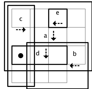
Figure 66 A sparse version of the optimal policy for the cockroach robot world, with five rules ( a..e ). Compare to Figure 63. The state marked \bullet is covered by three different rules ( a, c , and d ), with d being the most specific.
